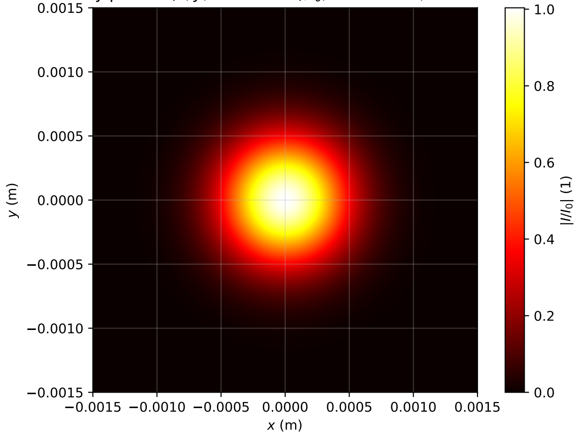
Intensity profile I(x, y, z = 0.159m)/I_0 , Pin=0.4Pcr, artificial time
